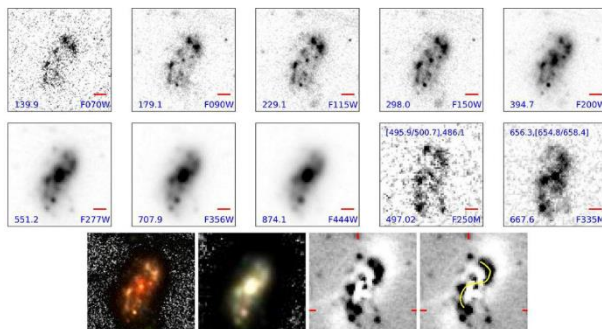
Grayscale cutouts of Alaknanda in all JWST broadband filters (top two rows). The red horizontal bar in the bottom right corner shows a 6,500-lightyear scale at the galaxy's redshift. The bottom row shows two composite images of the galaxy; the last two images show an algorithm's fitting of the telescope data. AA, 703 (2023) A&E.
