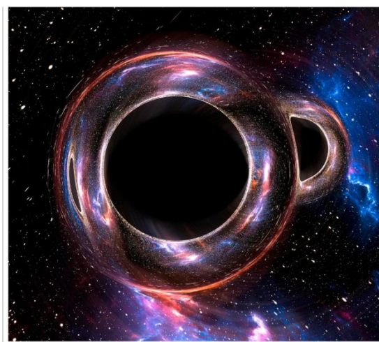
Artwork of a pair of merging black holes with differing masses. The gravity of the black holes bends and twists light around them. CAILIYONG, SQUARE, SHENYANG UNIVERSITY OF TECHNOLOGY
